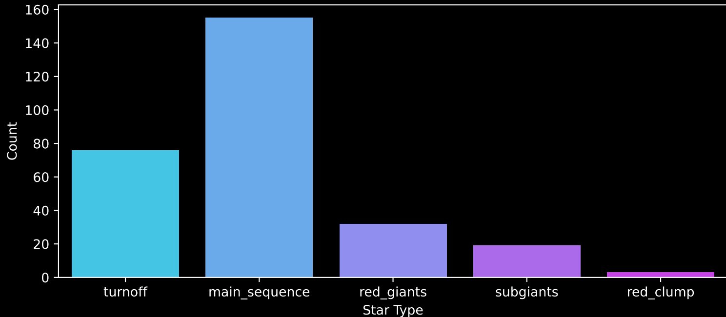
GALAH DR4 Field: [886] Count plot of Star Type
