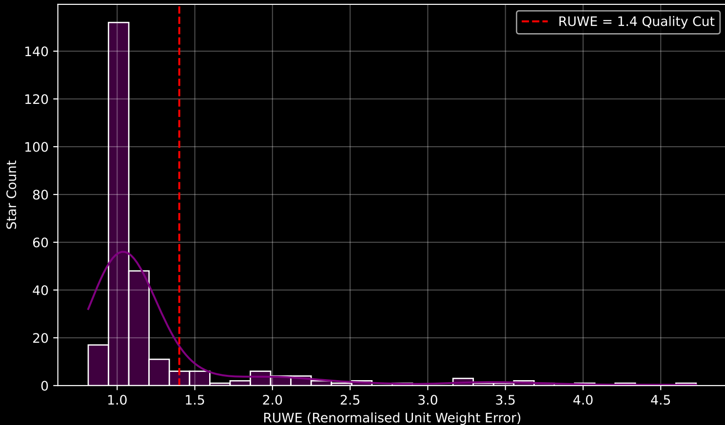
GALAH DR4 Field [886] RUWE Distribution (n= 274)
